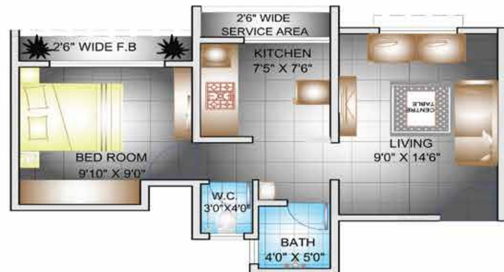
FLAT NO. - 103-603, 104-604 TYPICAL FLOOR PLAN, WING -A
